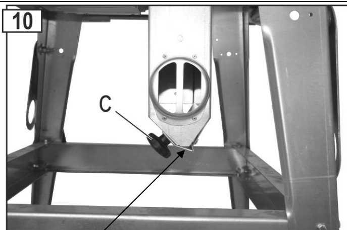
Chip ejector slot closed (operation with chip extractor)
