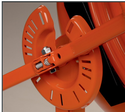
Ergonomic and smooth-running handwheel with multi ratch system for easy adjustment of the mixing drum.
