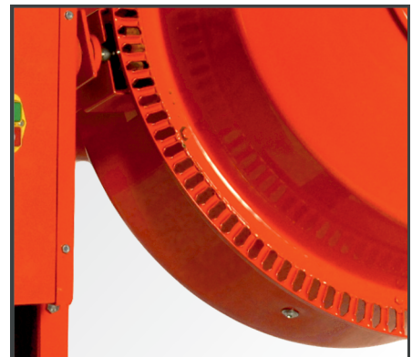
Break-proof gear rim made of sheet steel, drive pinion made of abrasion-resistant grey cast iron and powder coating for a long life.
