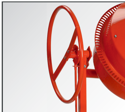
Large handwheel with ratchet disc & foot control for easy adjustment of the mixing drum.
