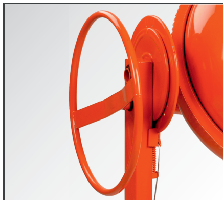
Large handwheel with smooth-running swing gear, disc brake & foot control for stepless adjustable mixing drum.
