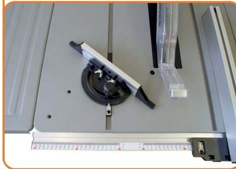
mitre fence and longitudinal stop
